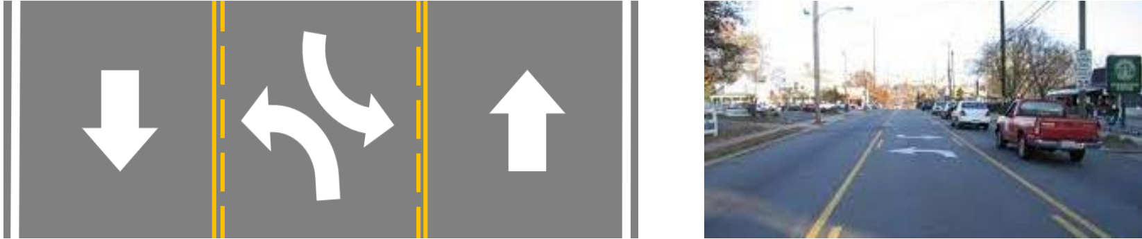
Figure 2: Three-lane (3T) Schematic and Example
