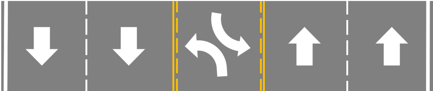
Figure 5: Five-lane Arterial (5T) Schematic and Example
