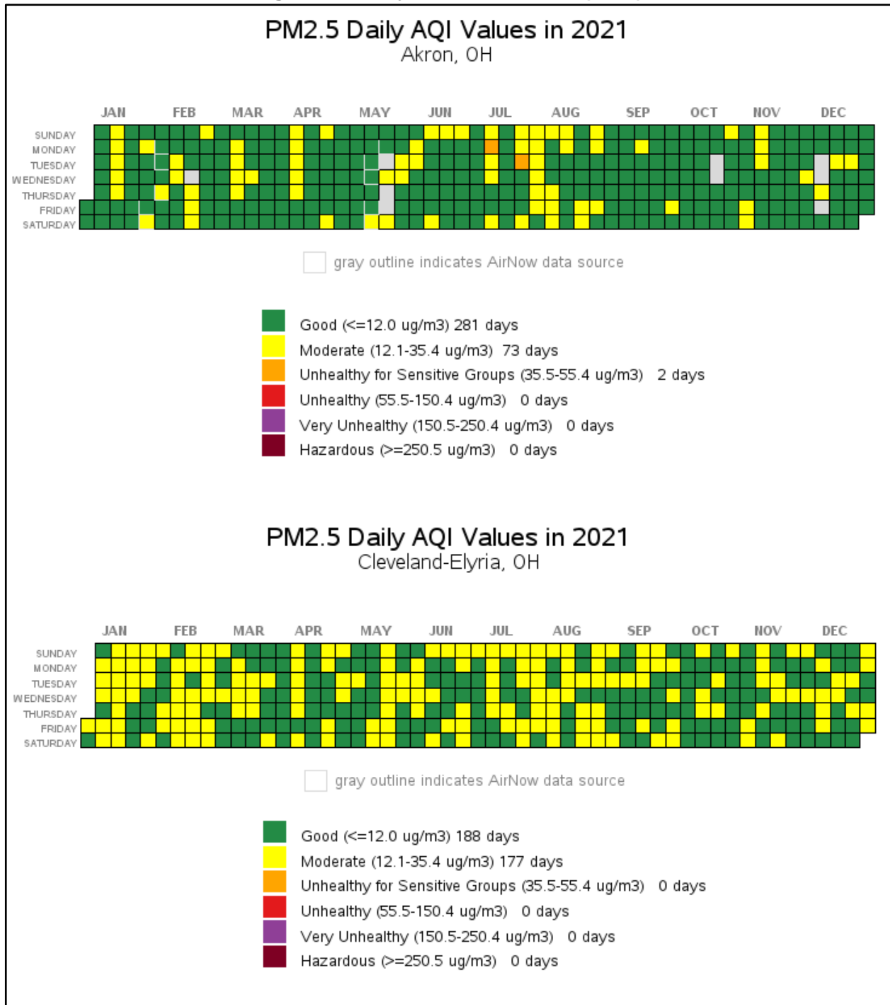
Figure 22: Daily PM 2.5 AQI Values (2021)
