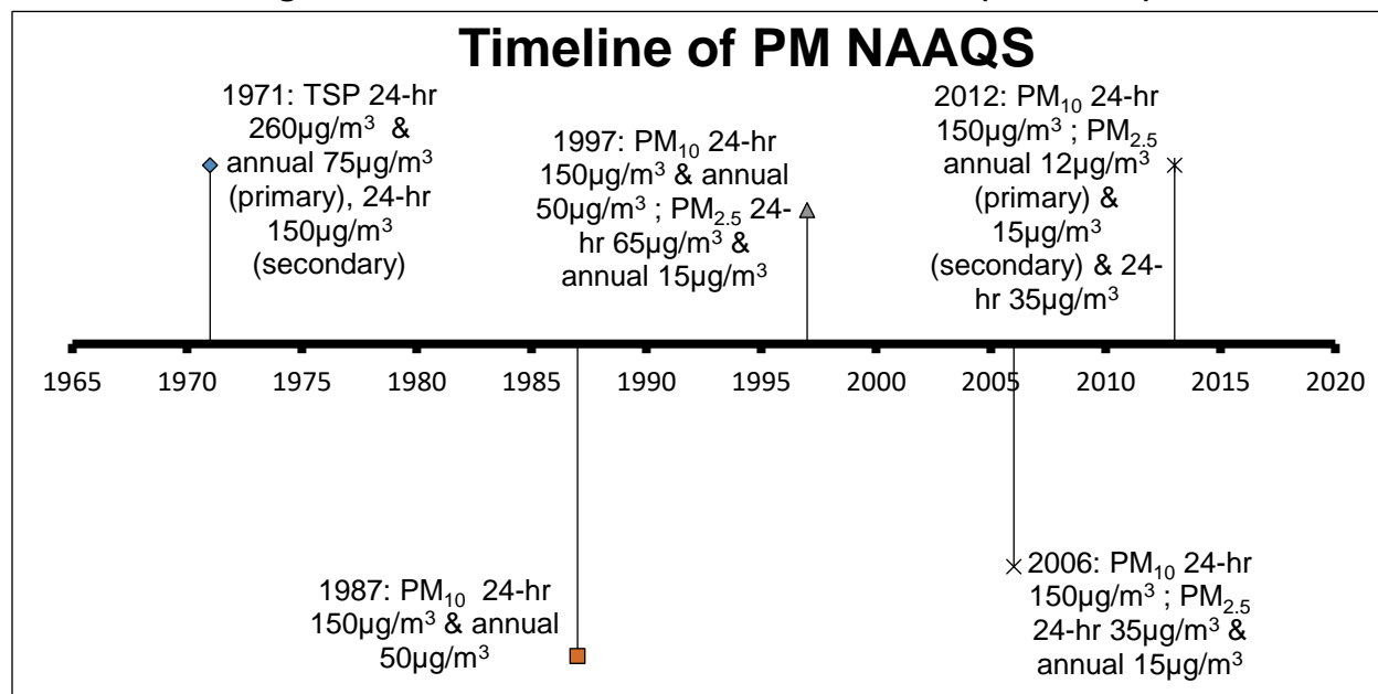
Figure 17: Timeline of Revisions to PM NAAQS (1971-2021)
