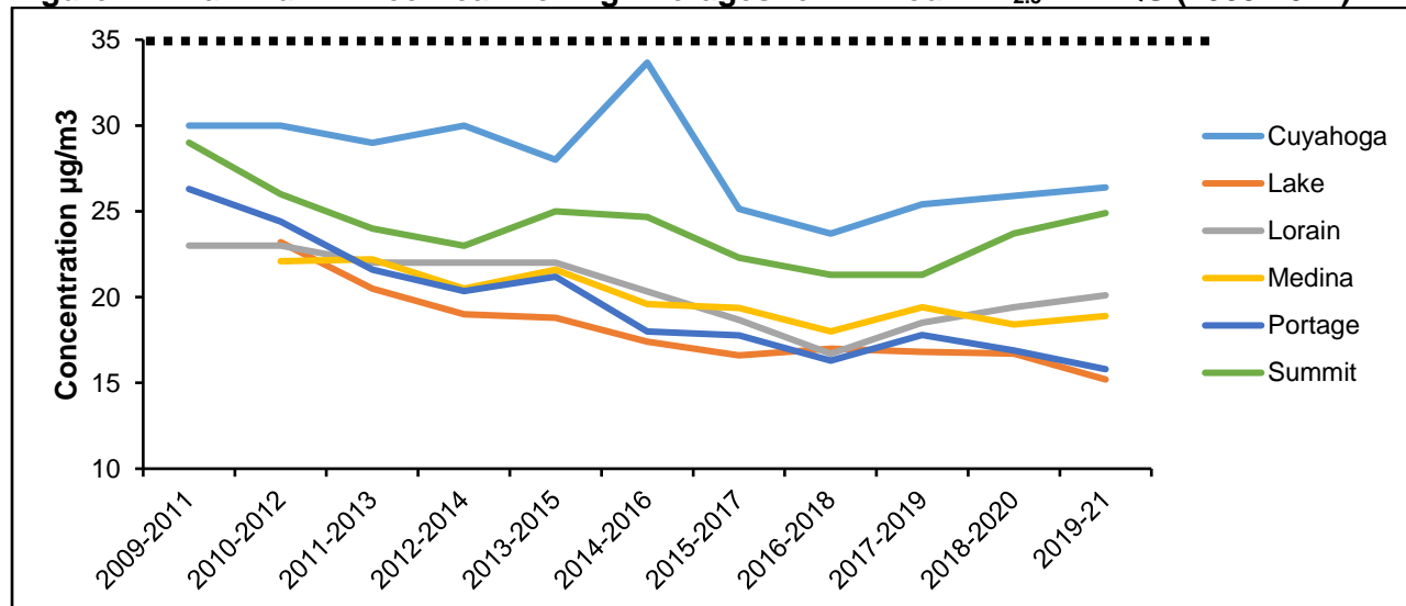
Figure 21: Maximum Three-Year Rolling Averages for 24-Hour PM_{2.5} NAAQS (2009-2021)
