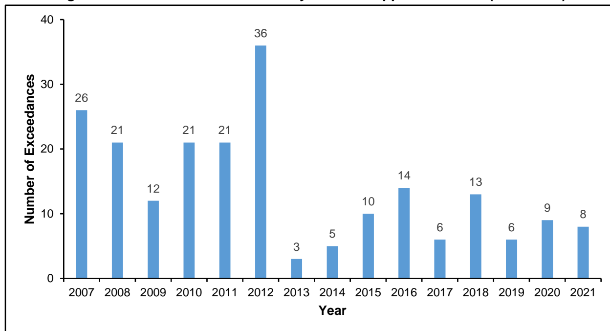
Figure 7: Number of Exceedance Days of the 70 ppb O 3 NAAQS (2007-2021)
