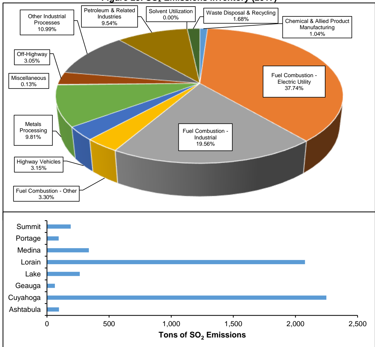
Figure 23: SO 2 Emissions Inventory (2017)
