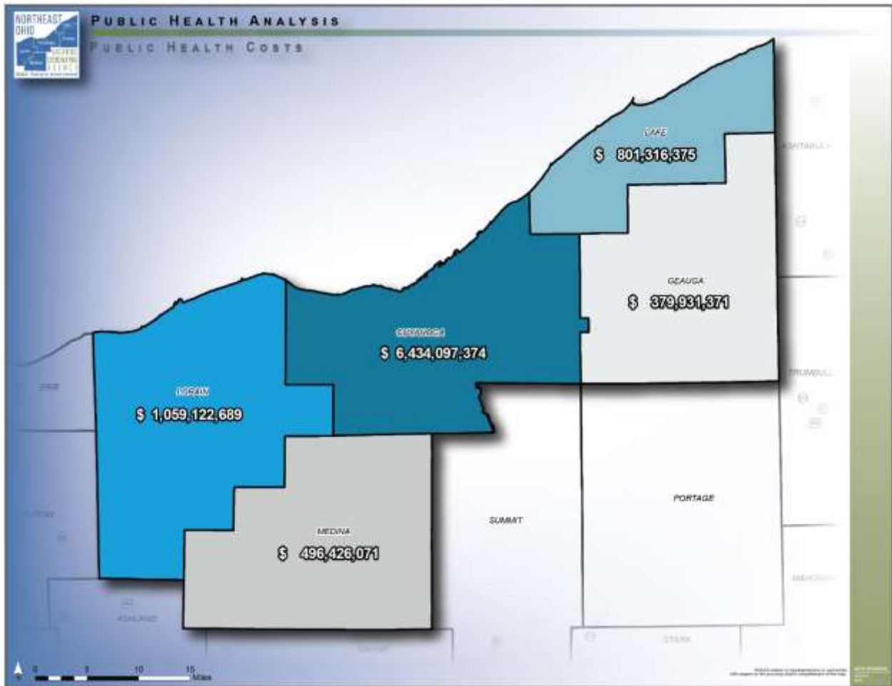
Figure 2: Distribution of Public Health Impacts of Air Pollutant Emissions in NOACA Region by County (2016)
