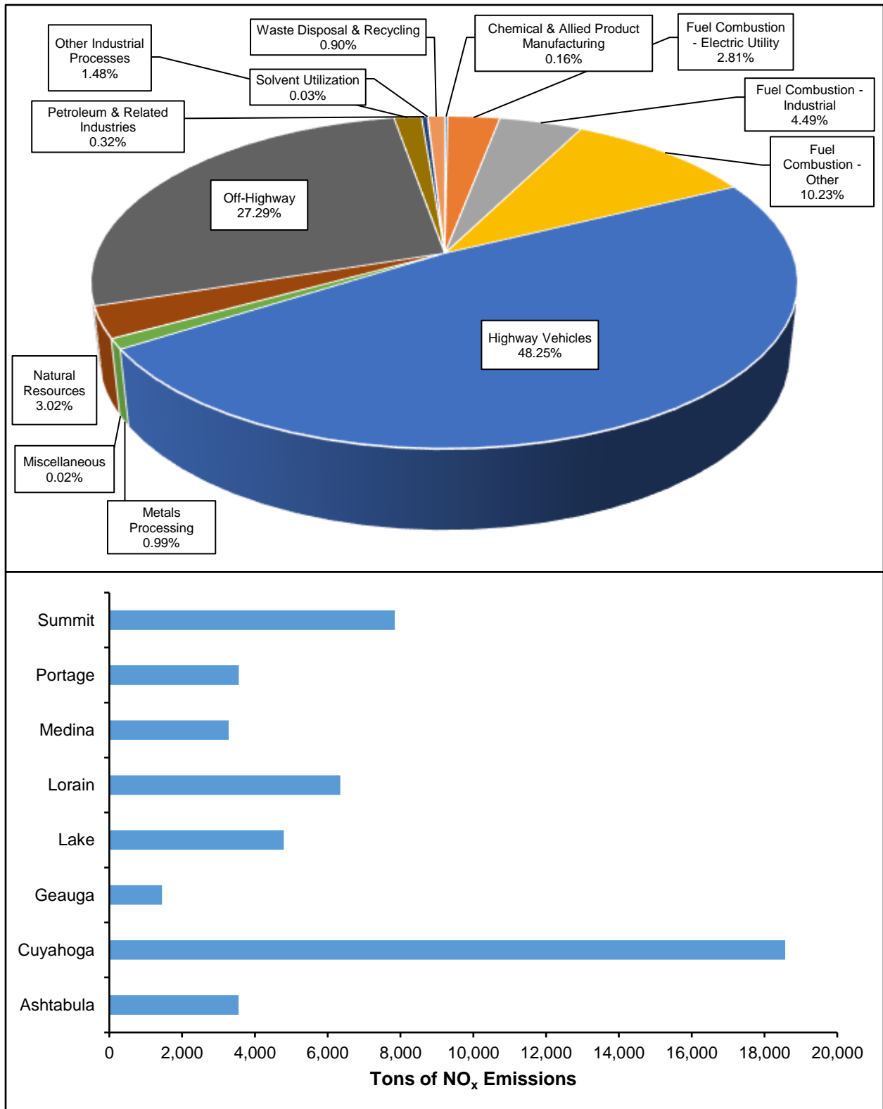
Figure 34: NO x Emissions Inventory for Northeast Ohio (2017)
