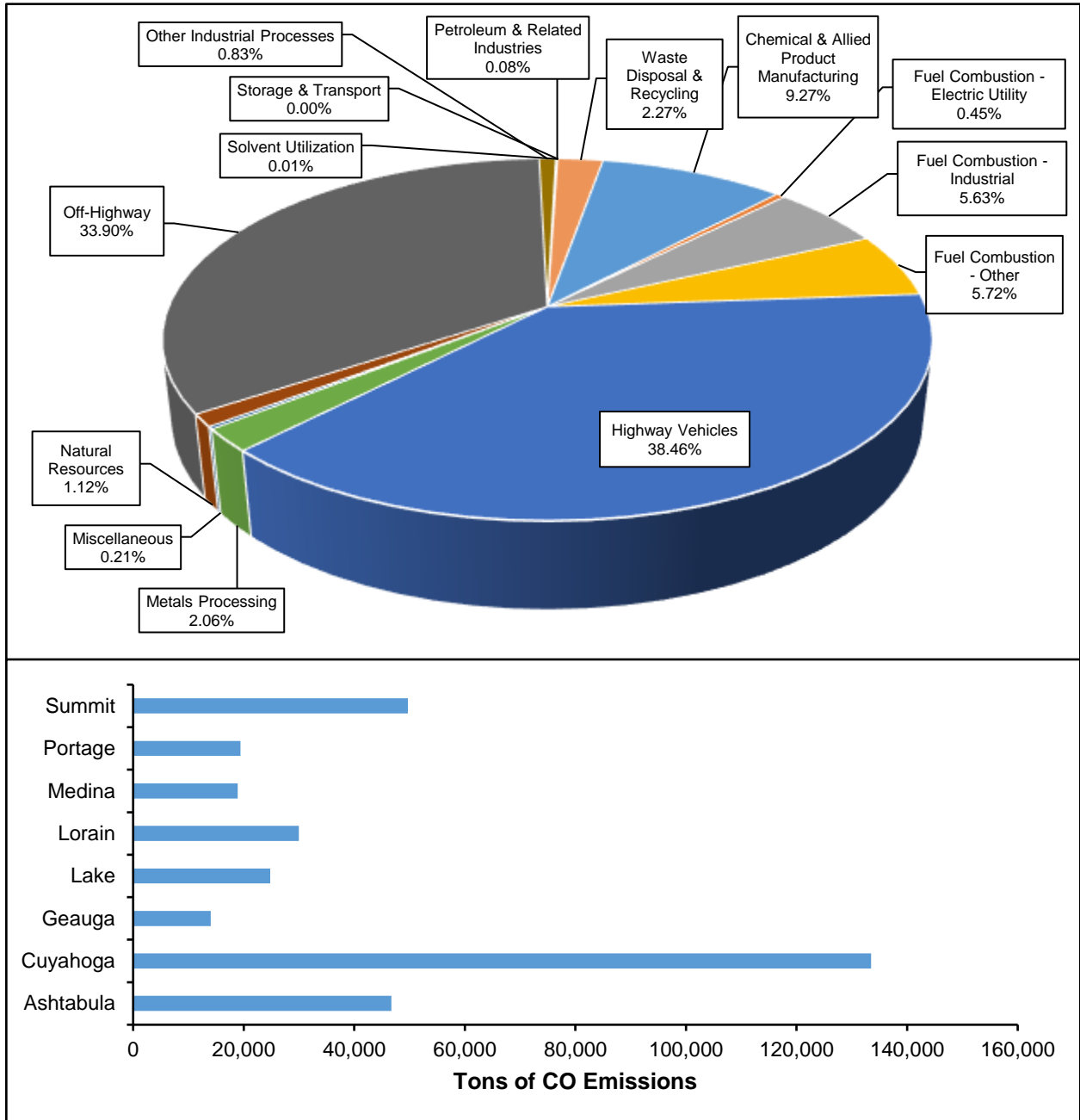
Figure 27: CO Emissions Inventory for Northeast Ohio (2017)
