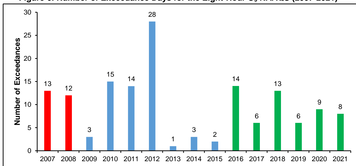
Figure 6: Number of Exceedance Days for the Eight-Hour O 3 NAAQS (2007-2021) 43
