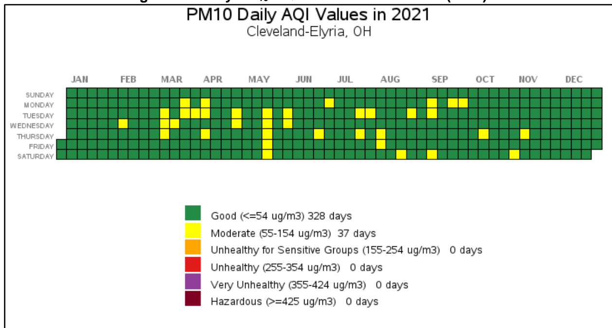
Figure 14: Daily PM 10 AQI Values for Cleveland (2021)
