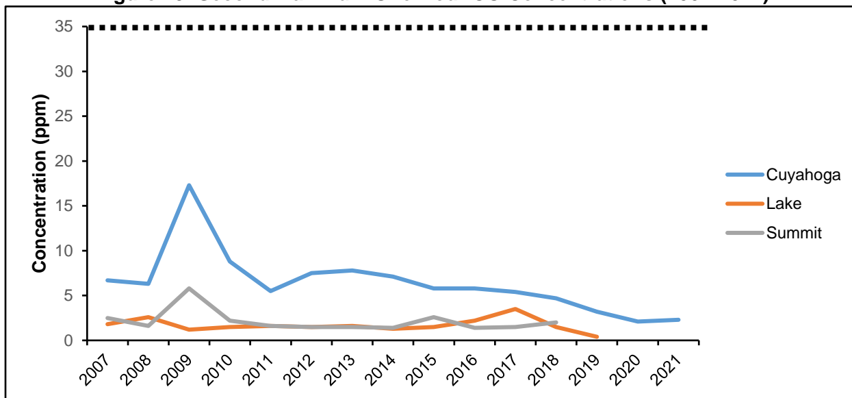
Figure 29: Second Maximum One-Hour CO Concentrations (2007-2021)
