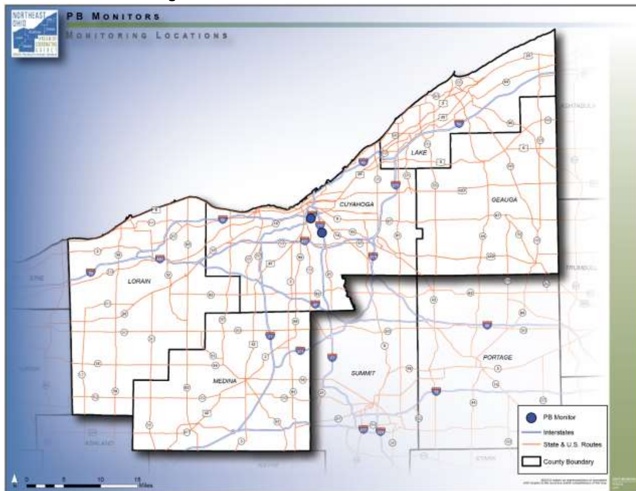
Figure 32: Northeast Ohio Pb Monitor Locations
