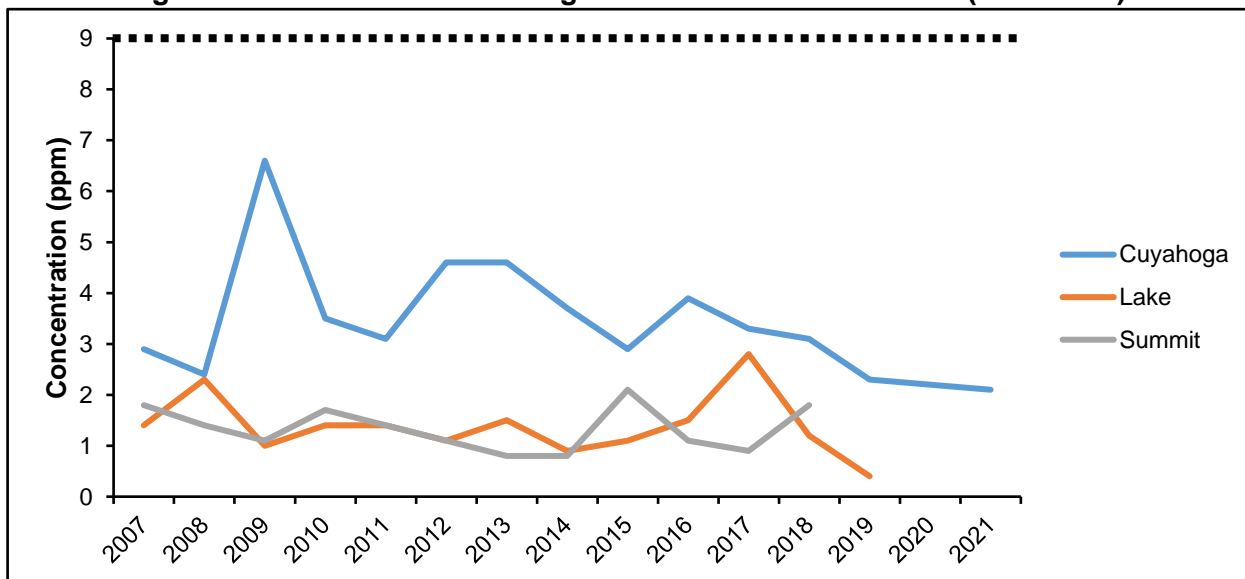
Figure 30: Second Maximum Eight-Hour CO Concentrations (2007-2021)
