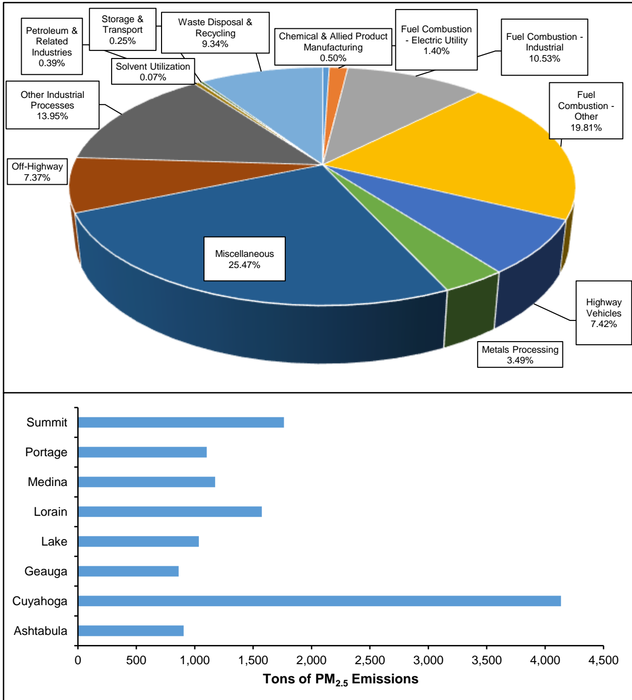
Figure 16: Primary PM 2.5 Emissions Inventory for Northeast Ohio (2017)
