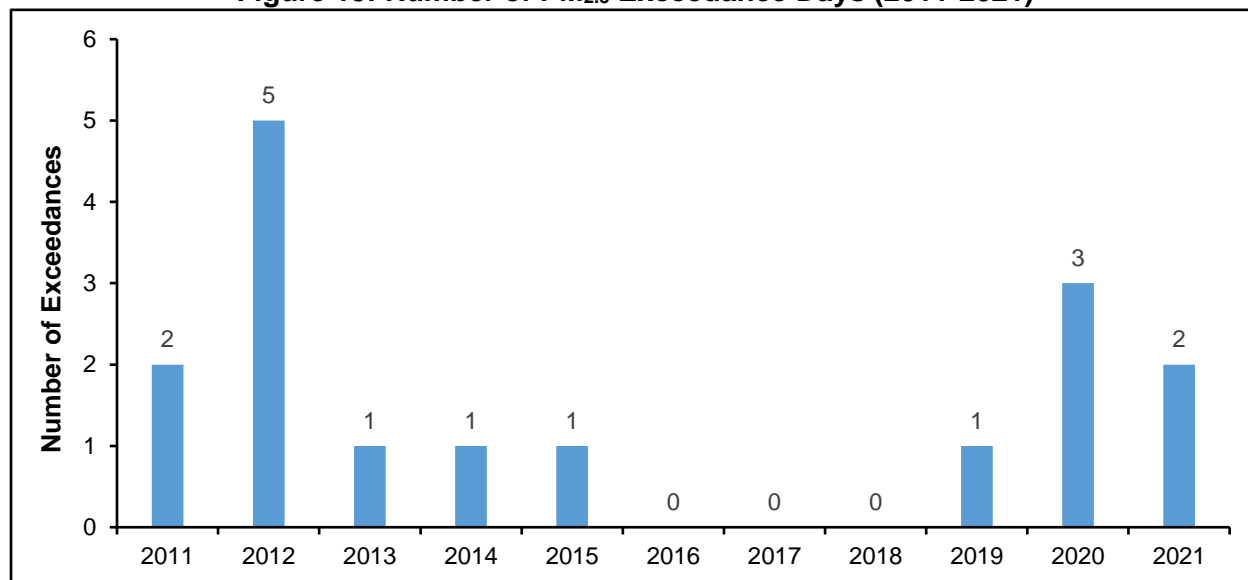
Figure 19: Number of PM 2.5 Exceedance Days (2011-2021)
