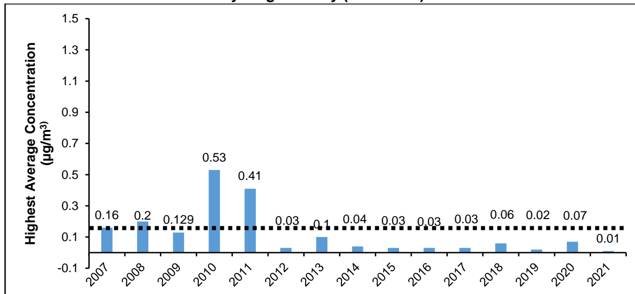
Figure 33: Highest Three-Month Average Pb Concentrations in Cuyahoga County (2007-2021) 56
