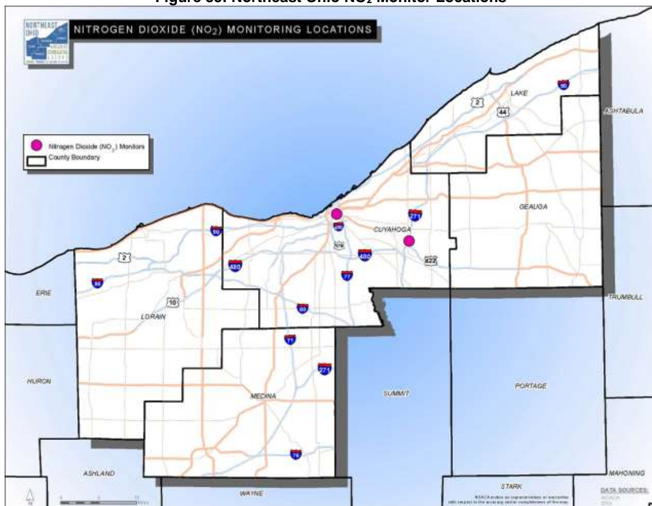
Figure 35: Northeast Ohio NO 2 Monitor Locations
