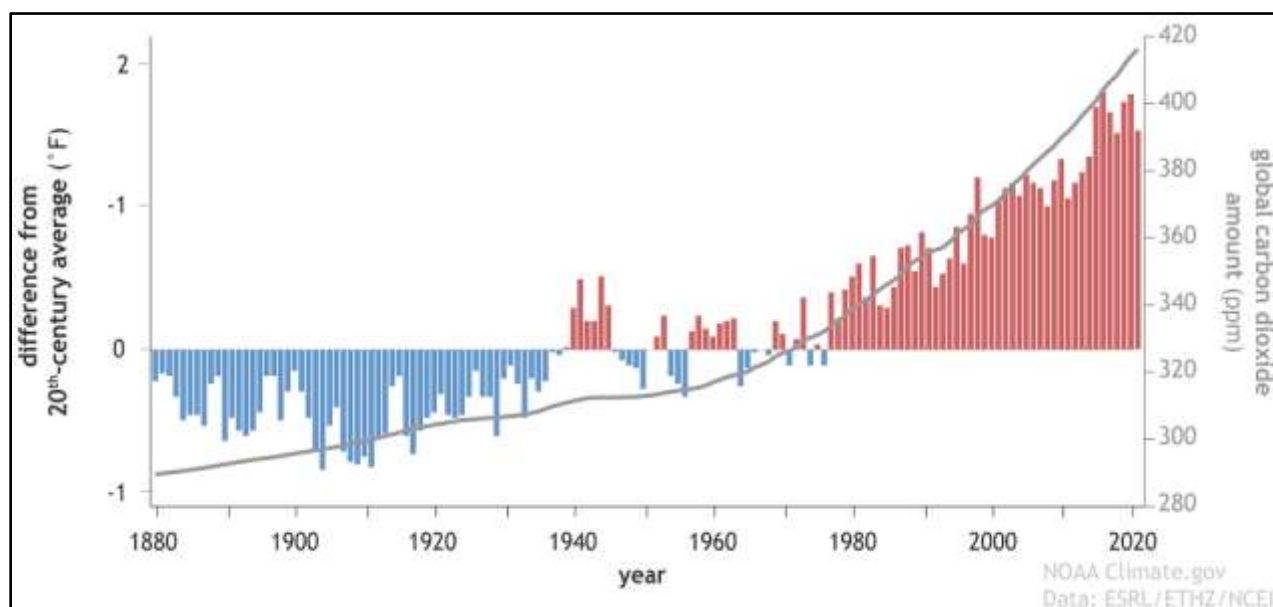
Figure 39: Atmospheric CO 2 and Earth's Surface Temperature (1880-2021)
