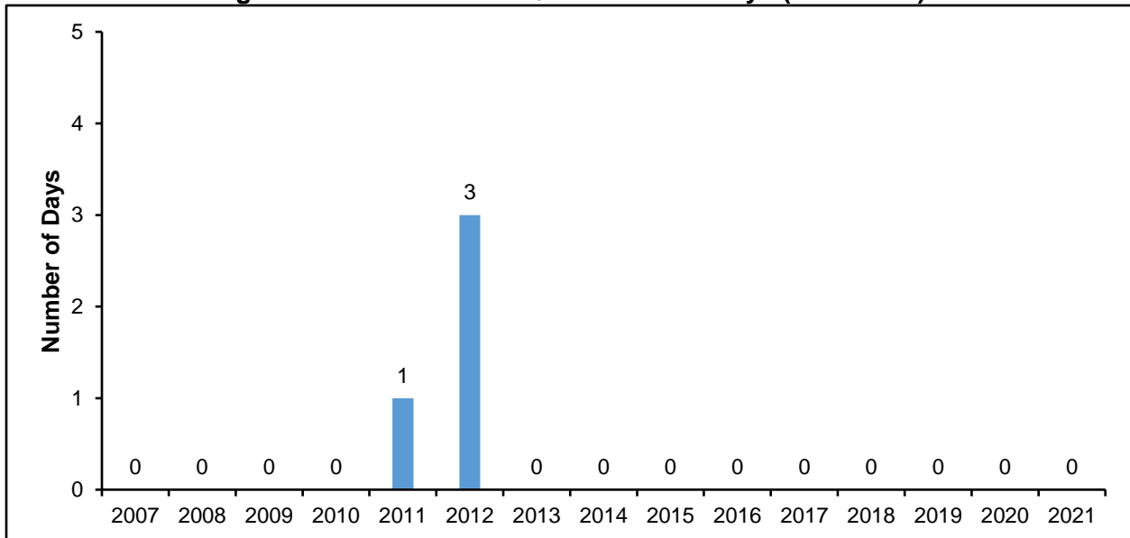
Figure 13: Number of PM 10 Exceedance Days (2007-2021)
