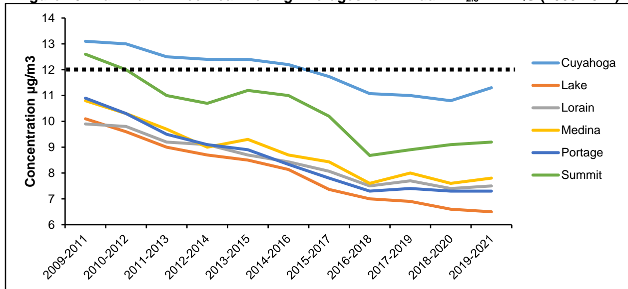
Figure 20: Maximum Three-Year Rolling Averages for Annual PM_{2.5} NAAQS (2009-2021) 49
