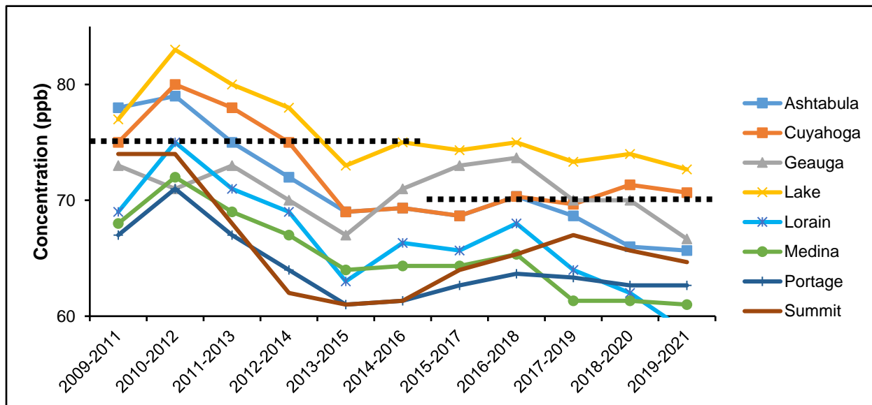
Figure 8: Rolling Three-Year O 3 Averages for Northeast Ohio (2009-2021) 47
