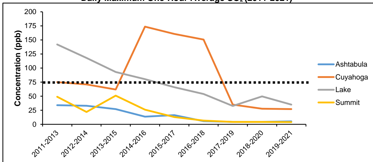
Figure 25: Three-Year Average of the 99th Percentile of Daily Maximum One-Hour Average SO 2 (2011-2021) 50
