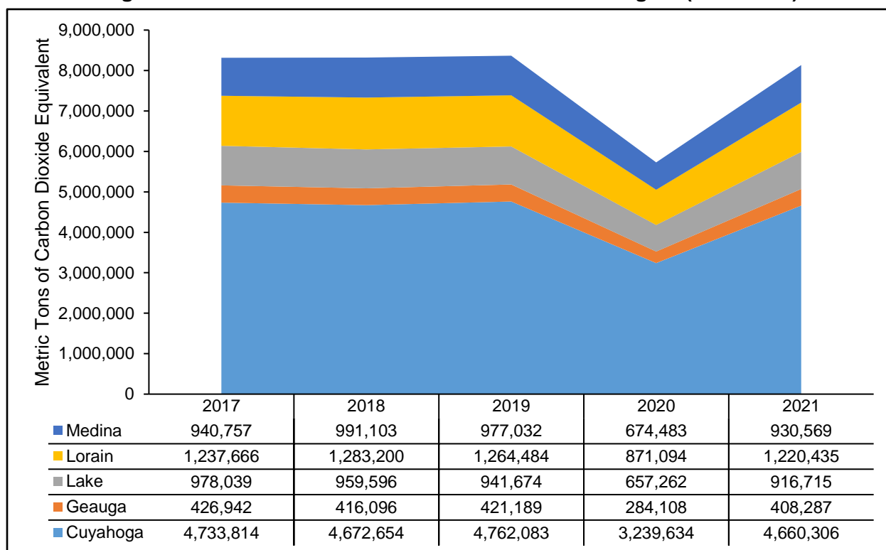
Figure 43: On-Road GHG Emissions in the NOACA Region (2017-2021)
