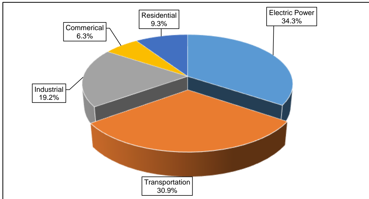
Figure 41: Share of GHG Emissions by Sector – Ohio
