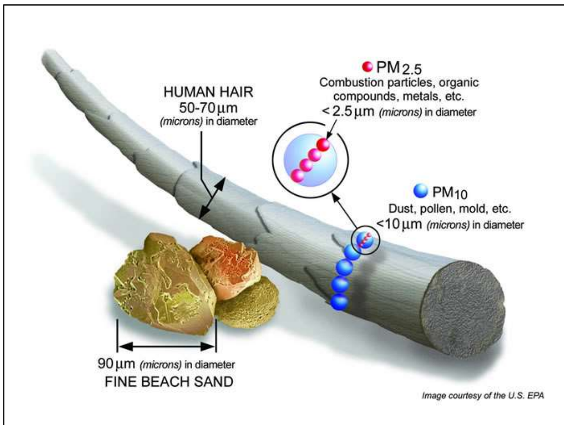
Figure 10: Particulate Matter Size
