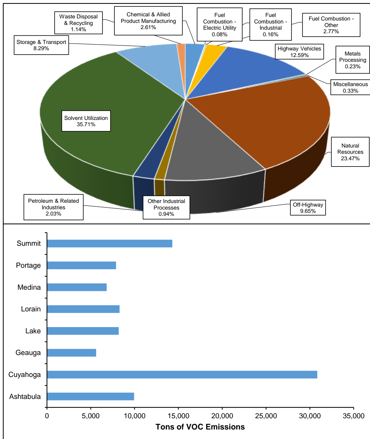
Figure 3: VOC Emissions Inventory for Northeast Ohio (2017)
