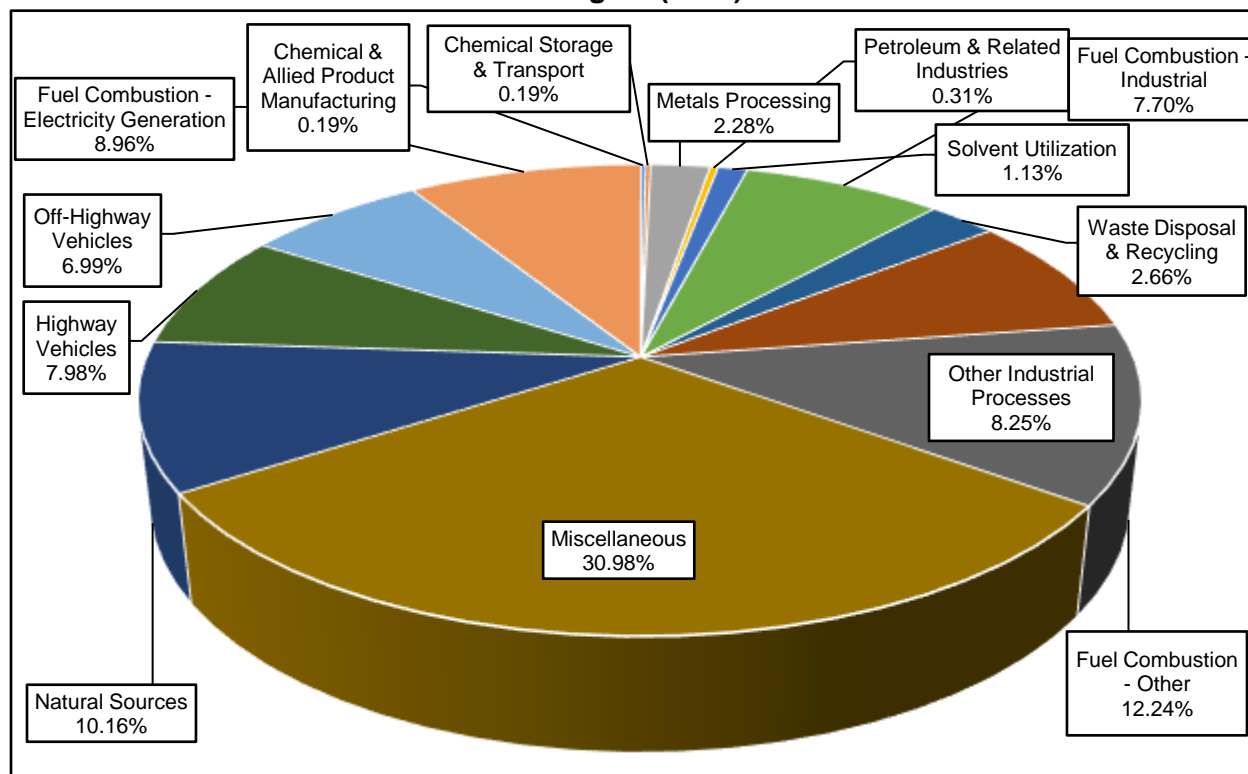
Figure 1: Share of Public Health Impacts from Air Pollutant Emissions by Sector in NOACA Region (2016)
