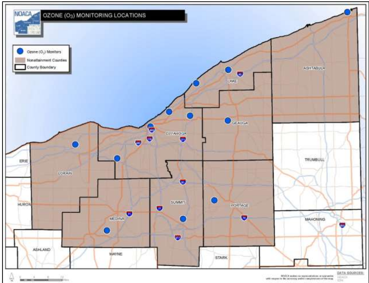
Figure 5: Northeast Ohio O 3 Monitor Locations
