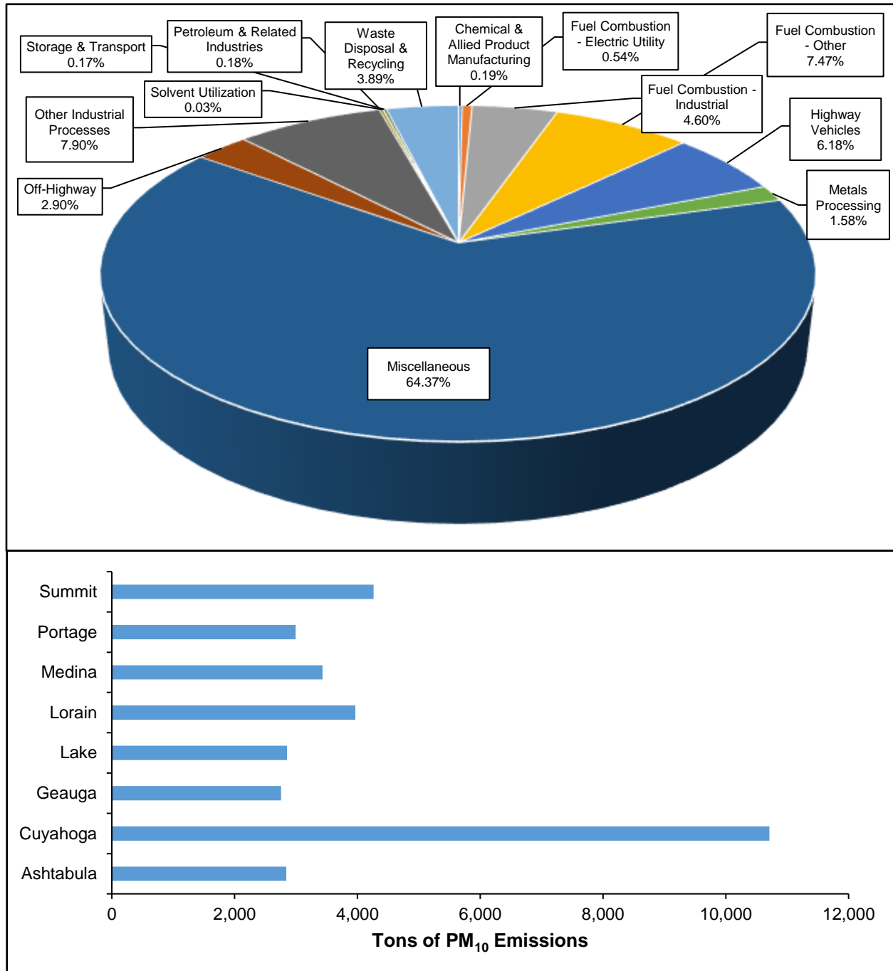
Figure 11: PM 10 Emission Inventory for Northeast Ohio (2017)
