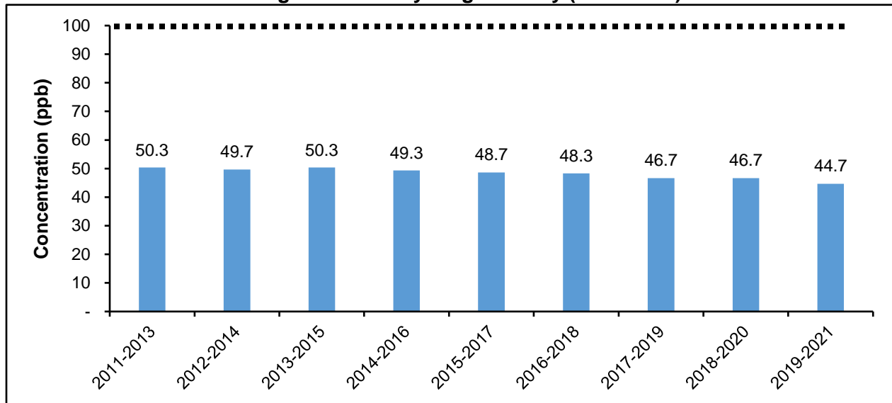
Figure 36: Three-Year Average of the 98th Percentile of the Daily Maximum One-Hour Average NO 2 for Cuyahoga County (2011-2021)
