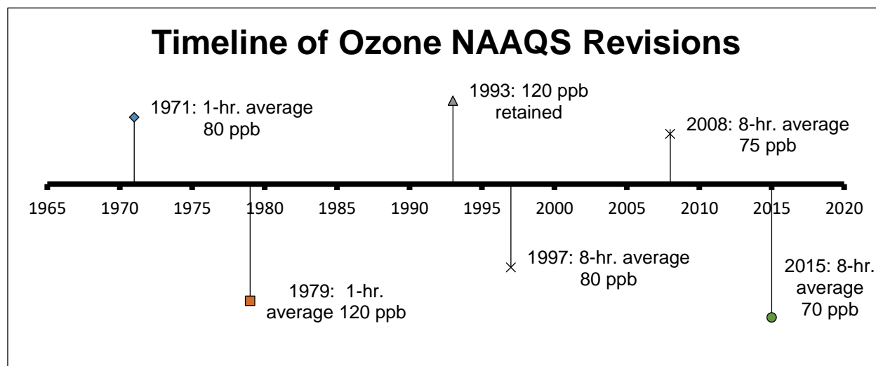
Figure 4: Timeline of Revisions to Ozone NAAQS (1971-2021)
