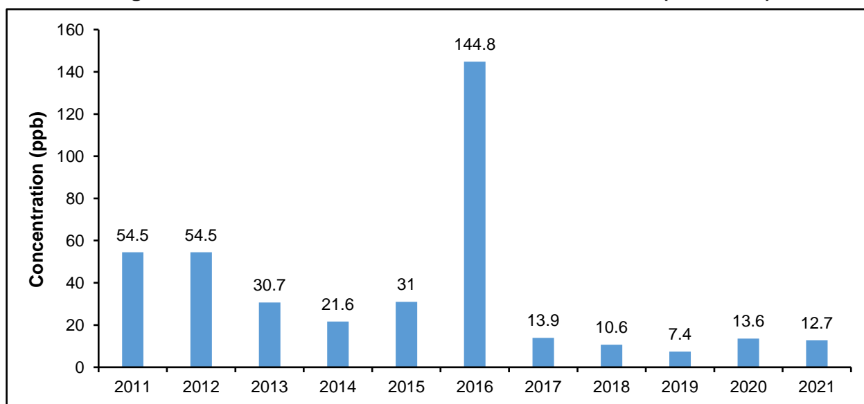
Figure 26: Second Maximum 24-Hour SO 2 Concentration (2011-2021)
