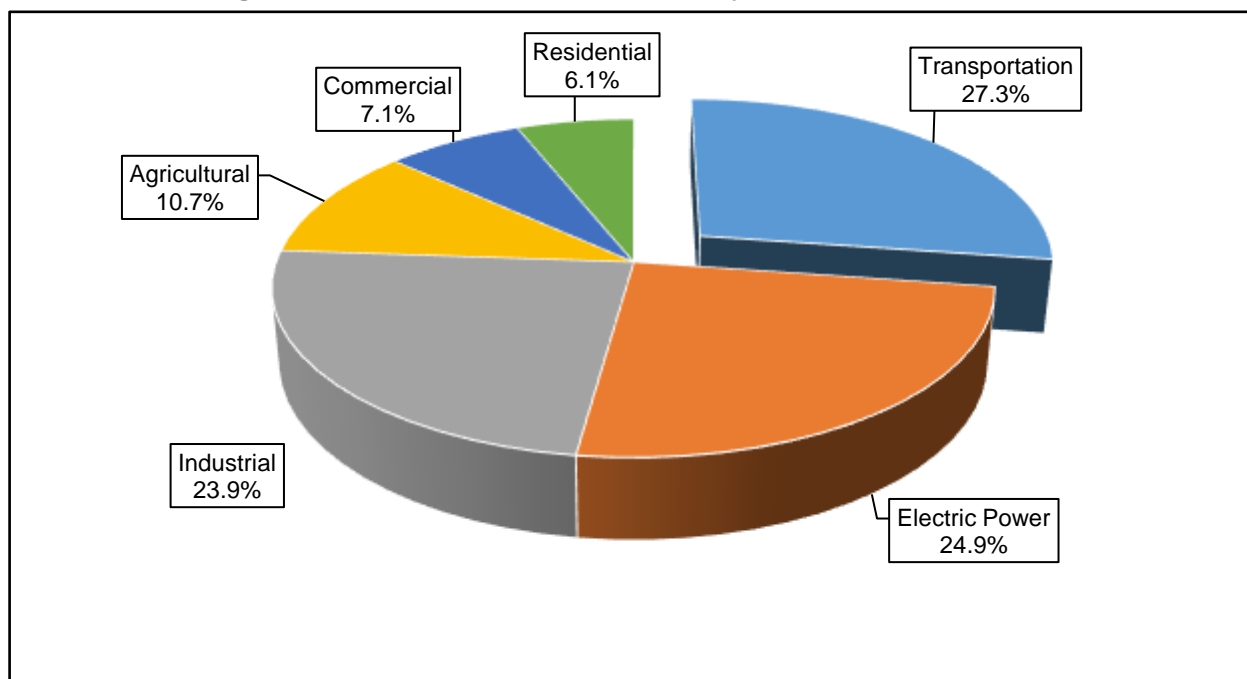
Figure 40: Share of GHG Emissions by Sector – United States
