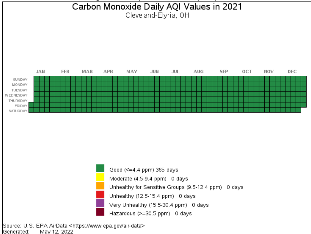
Figure 31: Daily CO AQI Values (2021) 53
