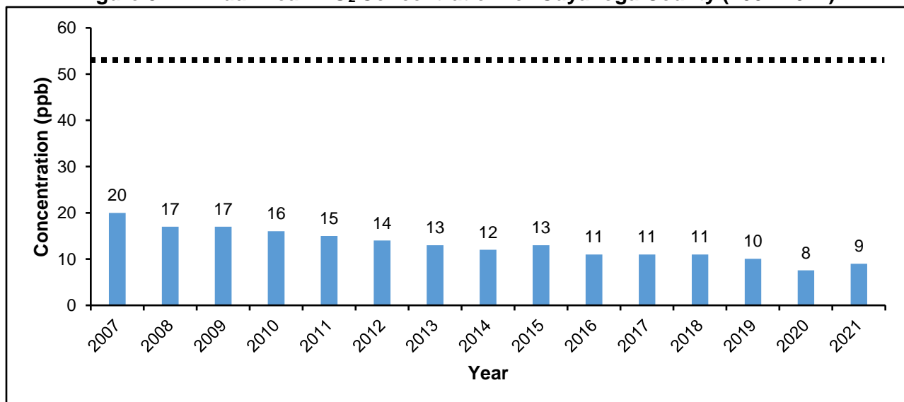
Figure 37: Annual Mean NO 2 Concentration for Cuyahoga County (2007-2021)
