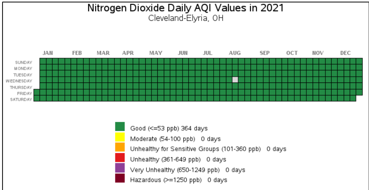
Figure 38: Daily NO 2 AQI Values (2021) 58
