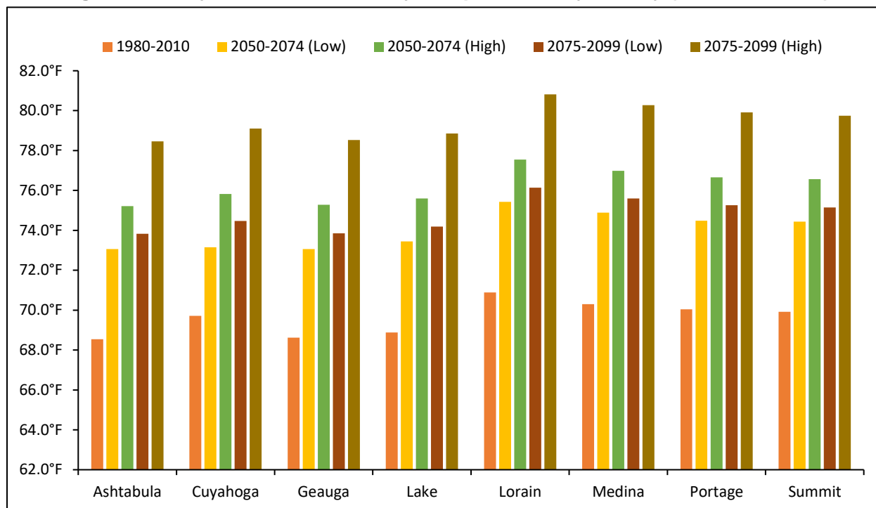
Figure 44: Projected Maximum Daily Temperatures by County (March-October)
