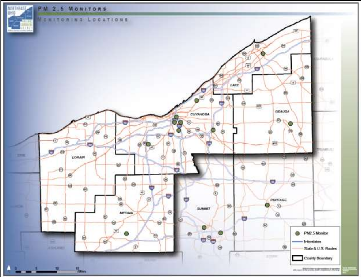
Figure 18: Northeast Ohio PM 2.5 Monitor Locations
