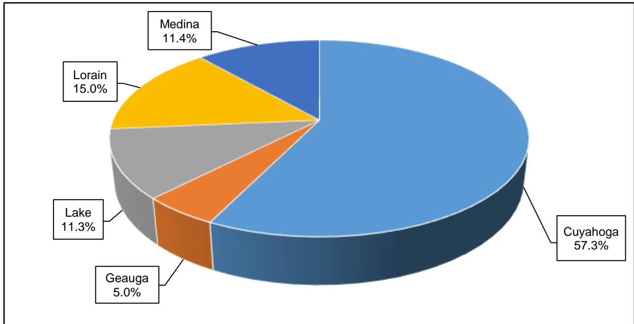
Figure 42: Share of On-Road GHG Emissions in Northeast Ohio by County (2021)
