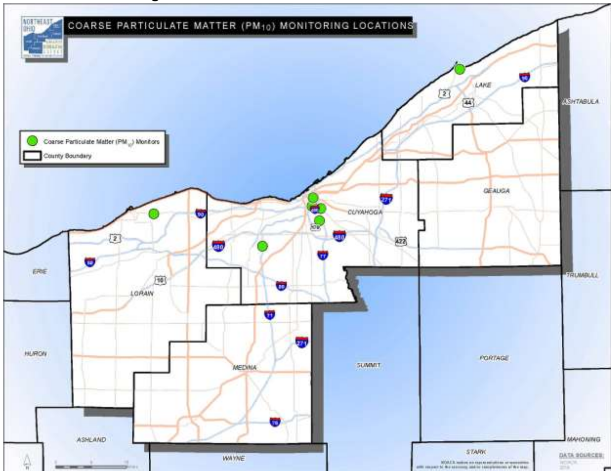
Figure 12: Northeast Ohio PM 10 Monitor Locations
